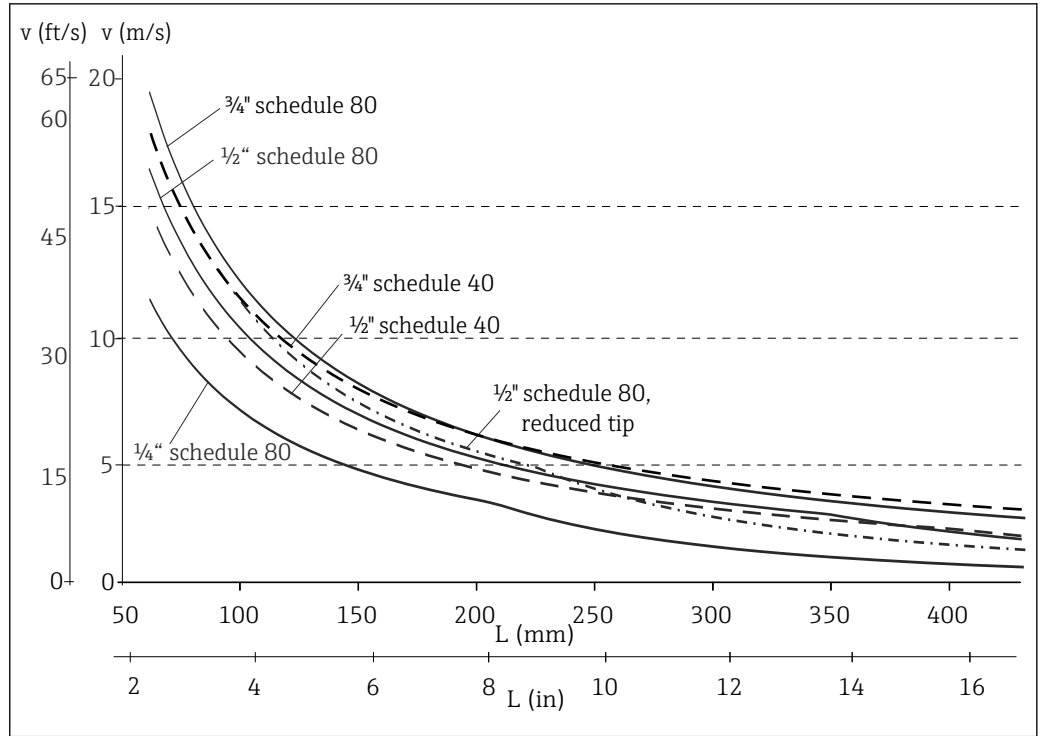
2 Permitted flow velocity with different thermometer diameters in the process medium water at T = 50\text{ }^{\circ}\text{C} ( 122\text{ }^{\circ}\text{F} )
