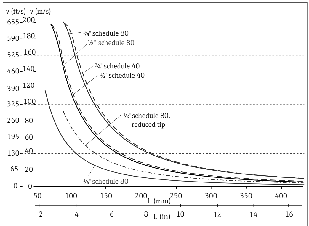
3 Permitted flow velocity with different thermometer diameters in the process medium superheated steam at T = 400\text{ }^{\circ}\text{C} ( 752\text{ }^{\circ}\text{F} )
