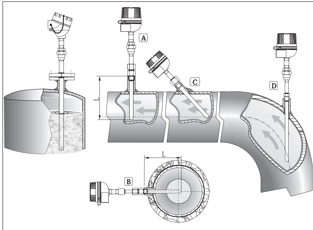
5 Installation examples
