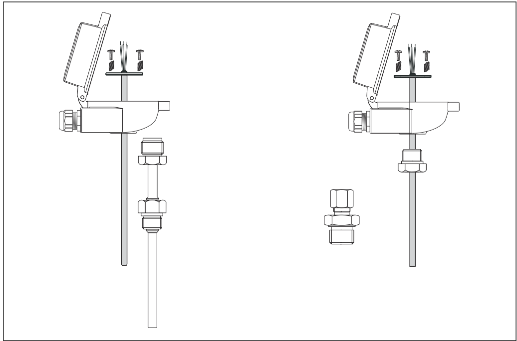
1 General installation options: in an assembly with thermowell (left), direct measurement (right)
