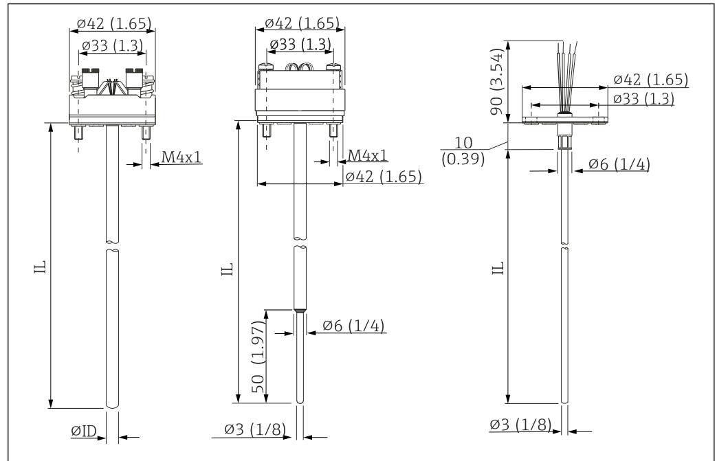
2 Design and dimensions of the TPR100
